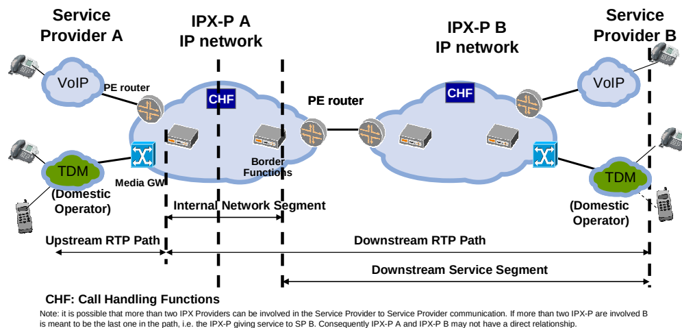
Figure 9 — Reference configuration for the IXP P-to-SP relationship
