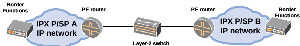
Figure 6 — Layer 2 Private-oriented Interconnection Configuration
