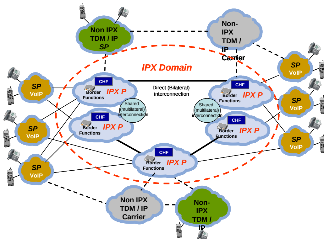
Figure 3 — Example IPX-network
