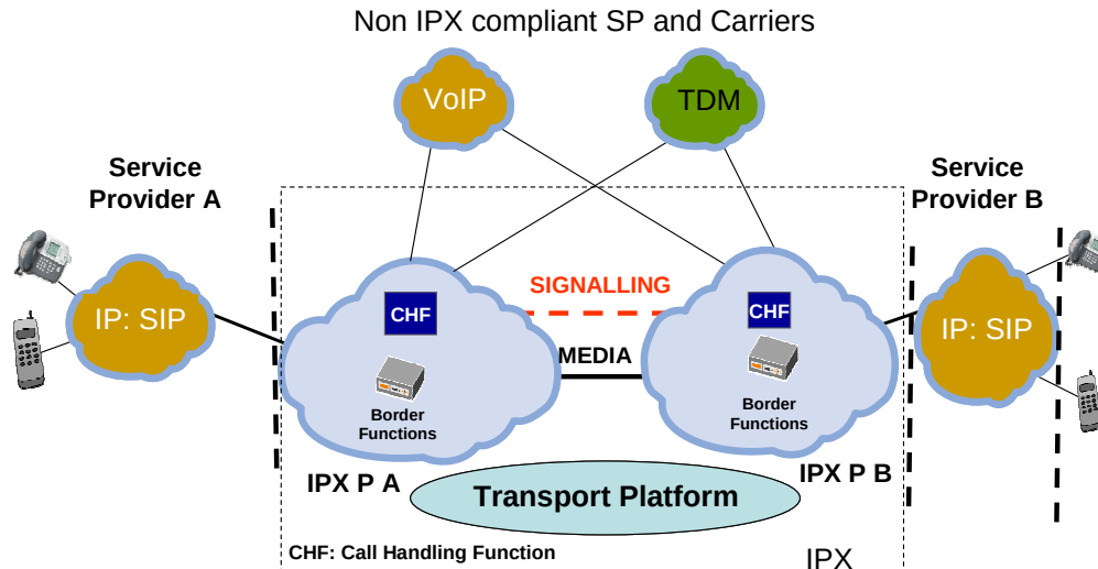
Figure 1 — General IPX Reference Configuration for Voice Services
