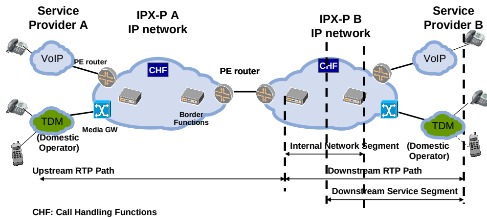
Figure 10 — Reference configuration for the IPX P-to-IPX P relationship
