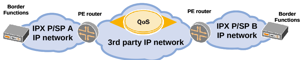
Figure 7 — Layer 3 Private-oriented Interconnection Configuration
