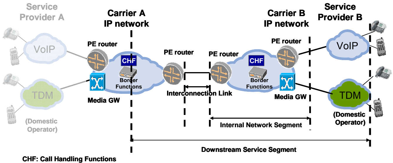
Figure 13 – Reference configuration for the Carrier-to-Carrier relationship
