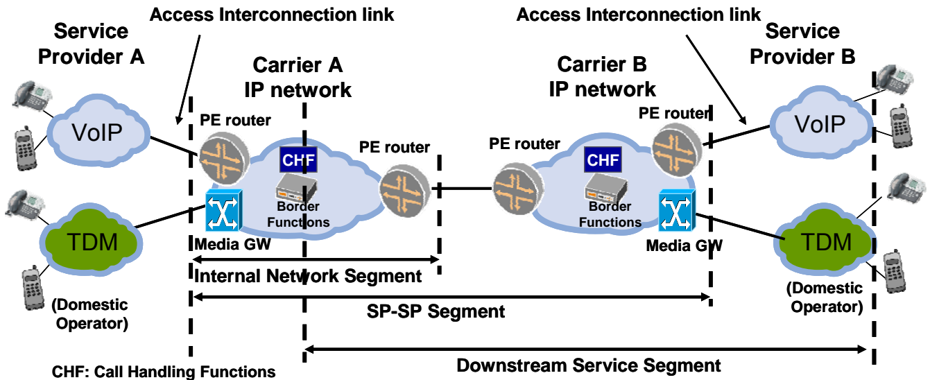
Figure 12 – Reference configuration for the Carrier-to-Service Provider relationship
