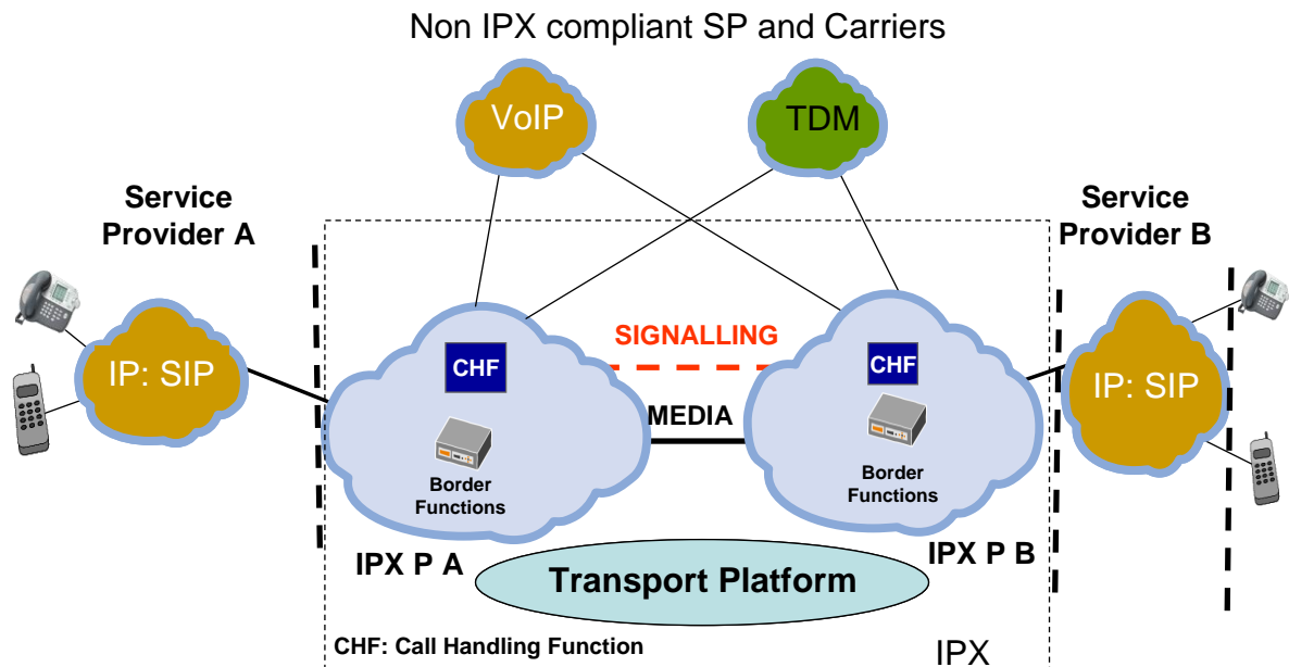
Figure 1 — General IPX Reference Configuration for Voice Services
