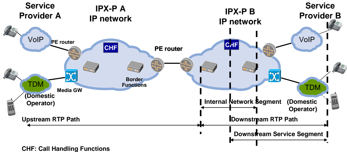
Figure 10 — Reference configuration for the IPX P-to-IPX P relationship
