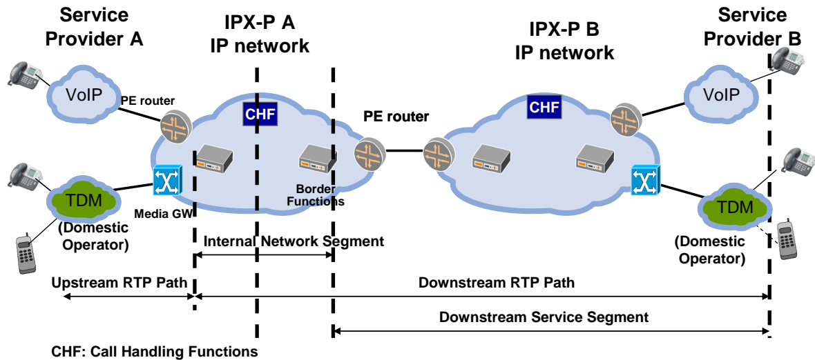
Figure 9 — Reference configuration for the IXP P-to-SP relationship
