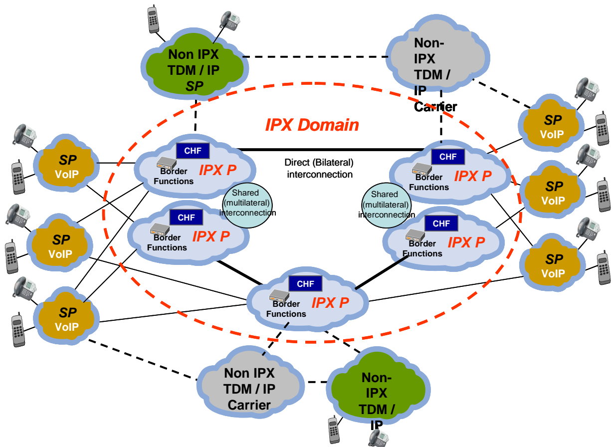
Figure 3 — Example IPX-network
