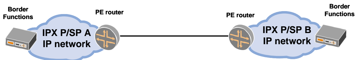
Figure 5 — Layer 1 Private-oriented Interconnection Configuration
